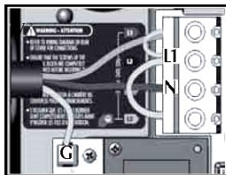
1-Phase
