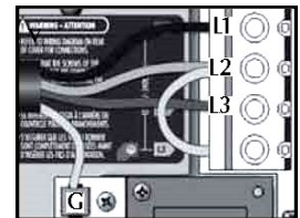
3-Phases Delta
